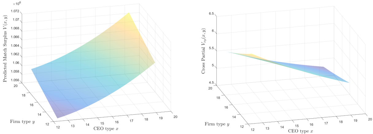
(a) The estimated expected match surplus V(x, y) (b) Complementarity of the match surplus V_{xy}(x, y)
